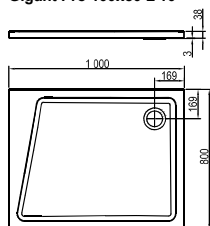
Gigant Pro 100x80 L 10°
