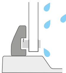
Raam dušinurga alumises osas: 10°, Nexty, Pivot, Blix Slim, Blix, Supernova
