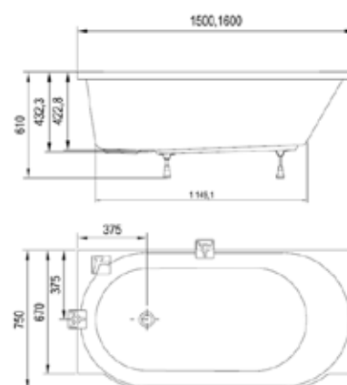
ARC 150/160 technical drawing
