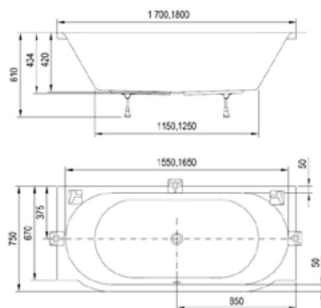
ARC 170/180 technical drawing
